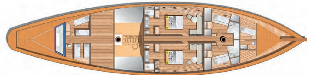
Lower Deck
